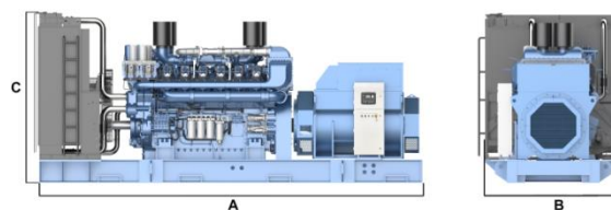
Open genset
